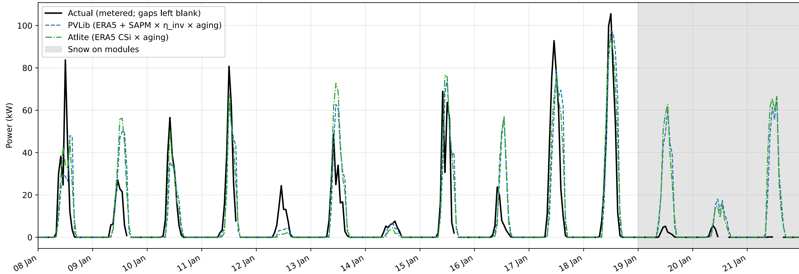
Campus Jülich PV, 8-21 January 2023 (matched ERA5; inverter/aging derates)
