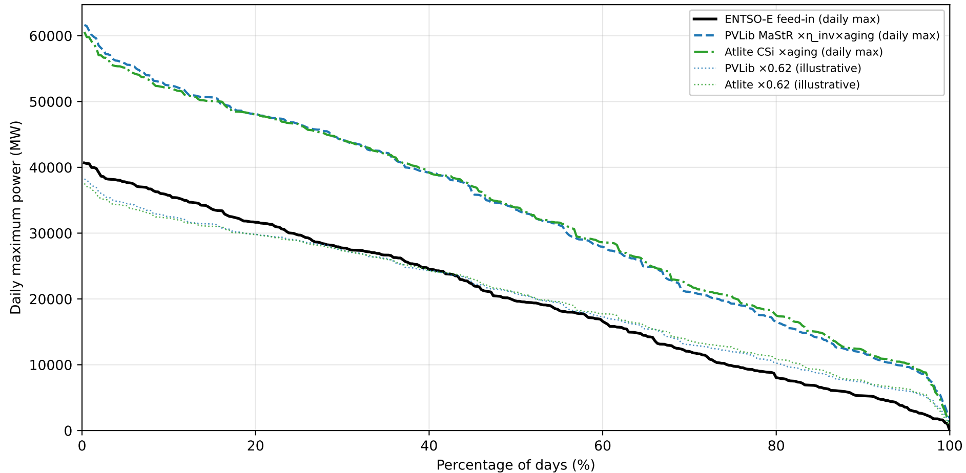
Germany national solar 2023 — duration curve of daily maximum (n=365 days; sims = generation after inverter/aging; ENTSO-E = public feed-in)
