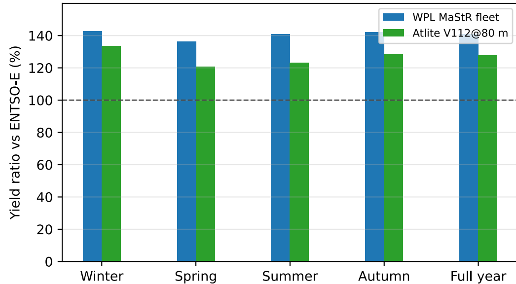
Onshore wind (fleet vs single-turbine proxy)
