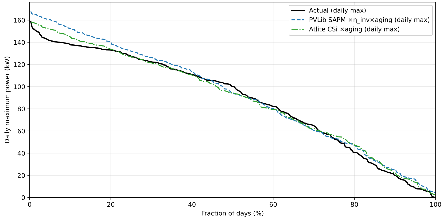
Jülich PV 2023 — duration curve of daily maximum generation (sims include inverter/aging)
