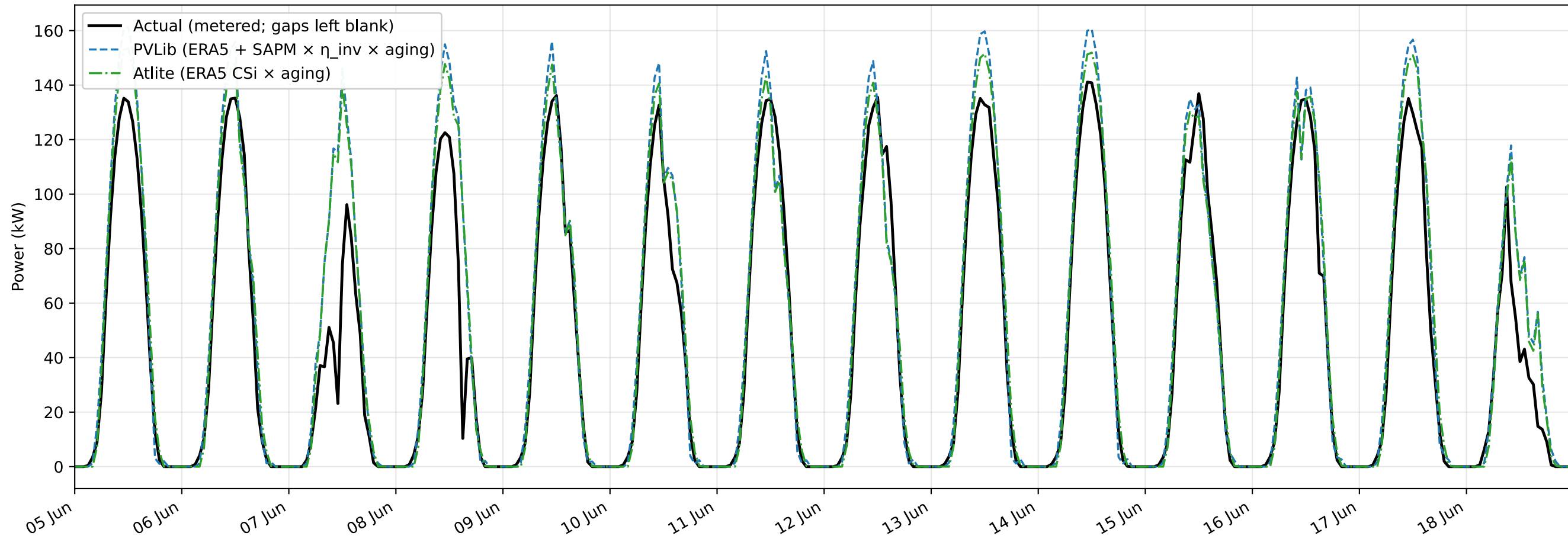
Campus Jülich PV, 5-18 June 2023 (matched ERA5; inverter/aging derates)
