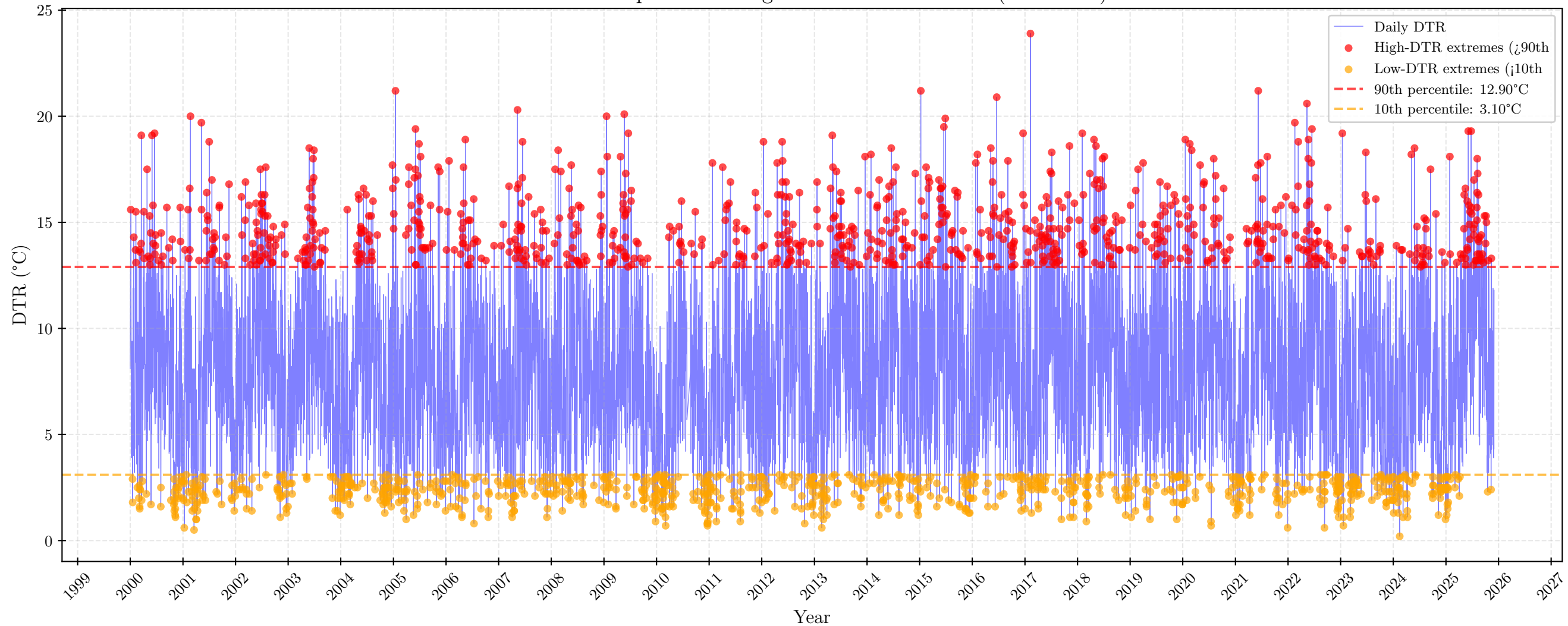
Diurnal Temperature Range with Extreme Events (2000-2025)
