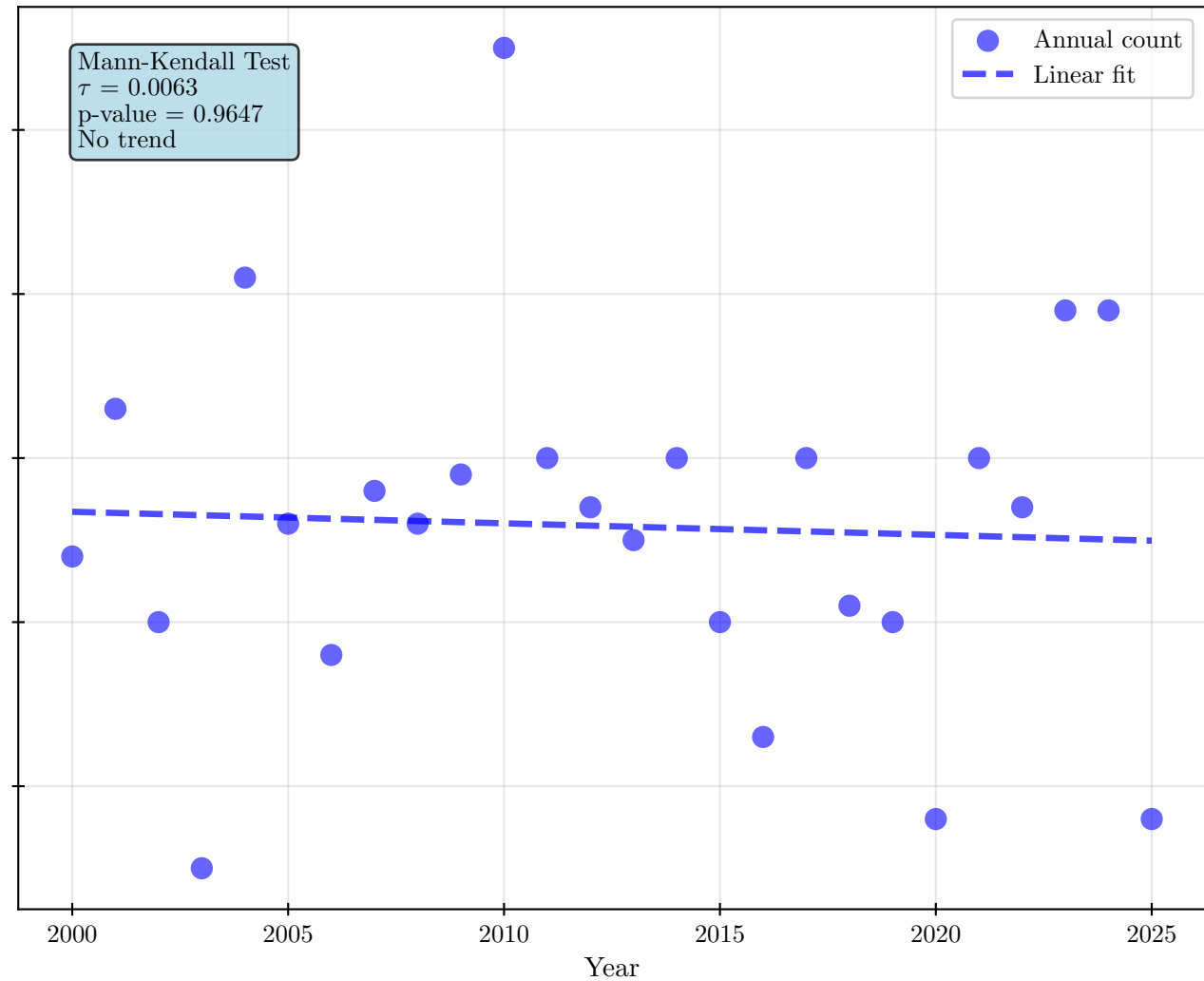
High-DTR Extreme Days per Year (90th percentile) Low-DTR Extreme Days per Year (10th percentile) DTR Extreme Event Trends (2000–2025): Mann-Kendall Analysis
