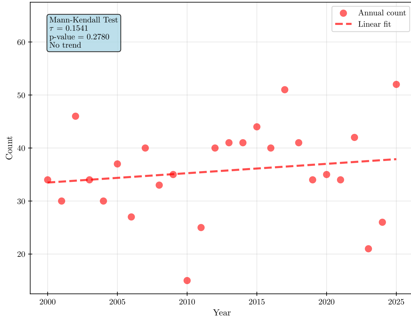
High-DTR Extreme Days per Year (90th percentile) Low-DTR Extreme Days per Year (10th percentile) DTR Extreme Event Trends (2000–2025): Mann-Kendall Analysis
