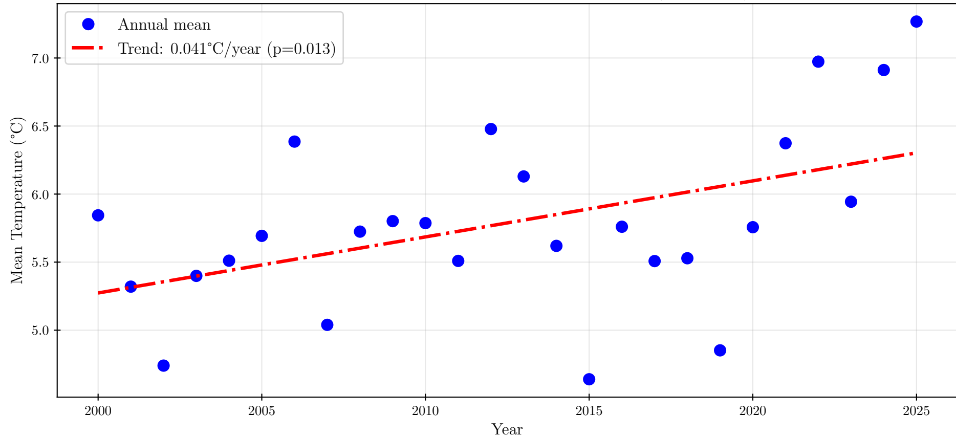
Annual Mean Temperature Trend in St. John's (2000-2025)
