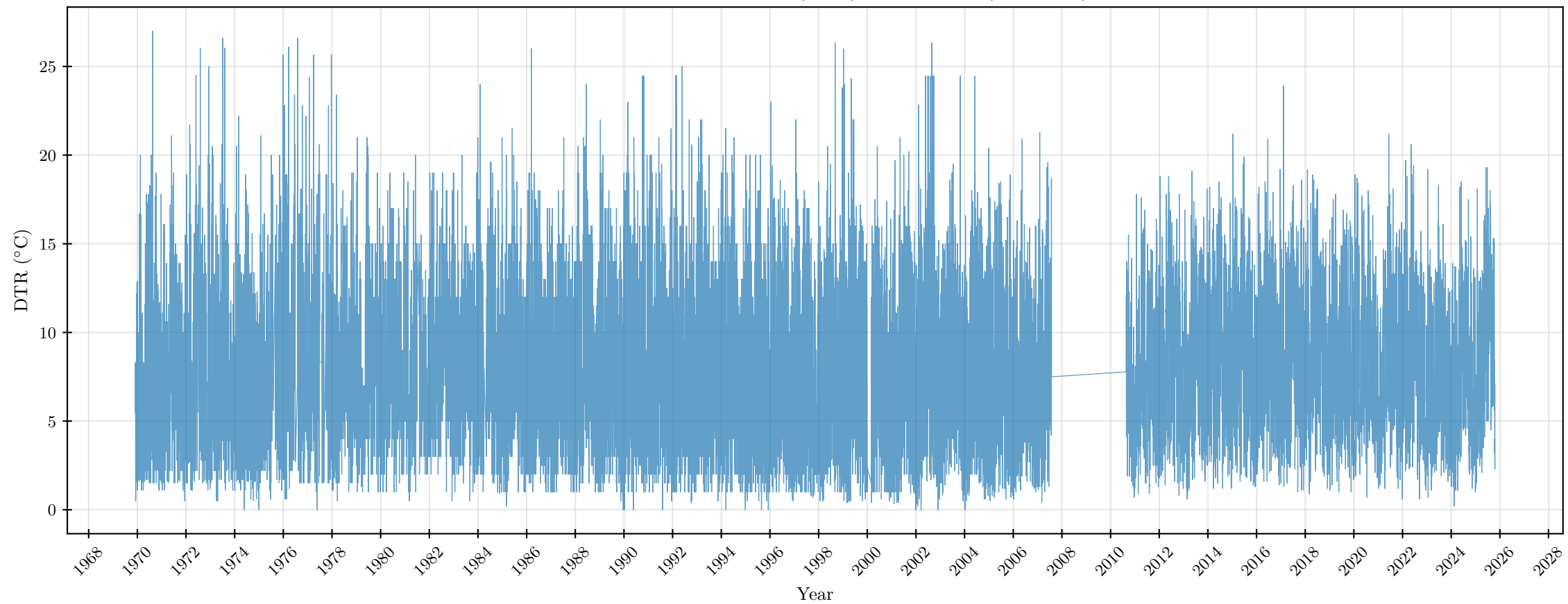
Diurnal Temperature Range (DTR) in St. John's (1969-2025)
