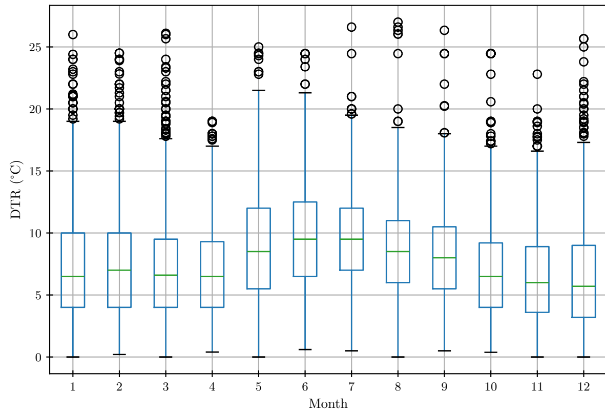
DTR Distribution by Month
