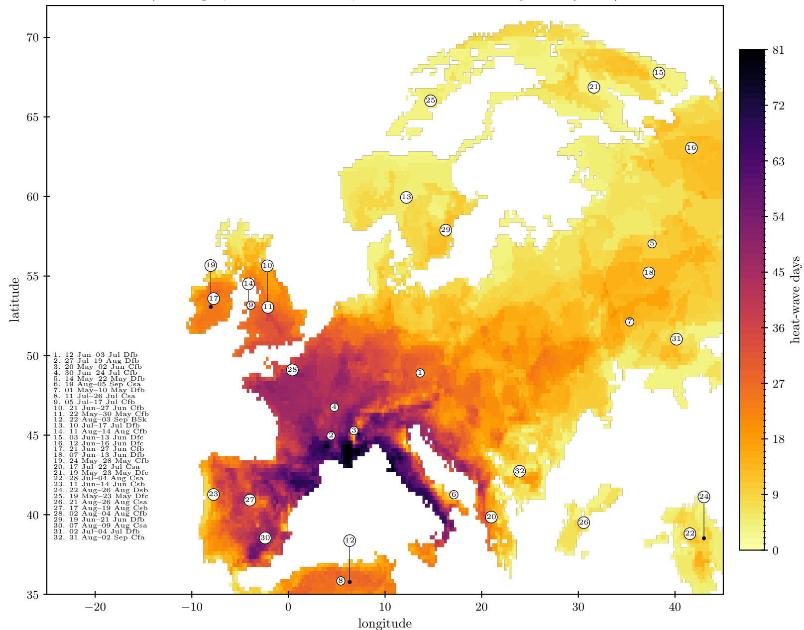
European heat waves 2026: days above the calendar-day 90th percentile (CTX90pct, 1991–2020 baseline; all 32 events numbered by severity rank)
