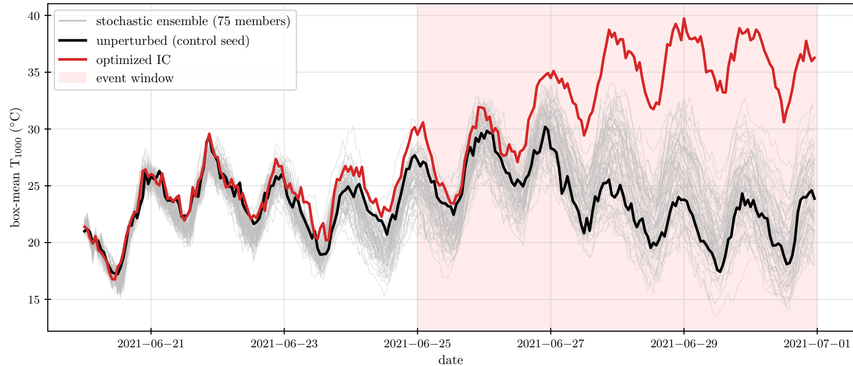
pnw_jun2021 storyline vs 75-member ensemble
