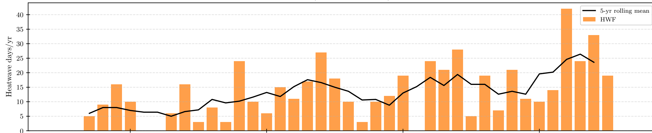
EHF (Excess Heat Factor)
