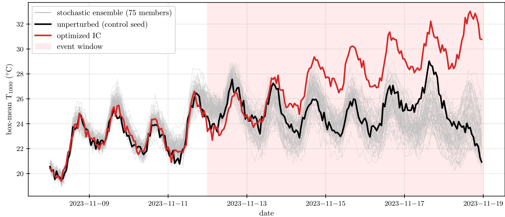
brazil_nov2023 storyline vs 75-member ensemble
