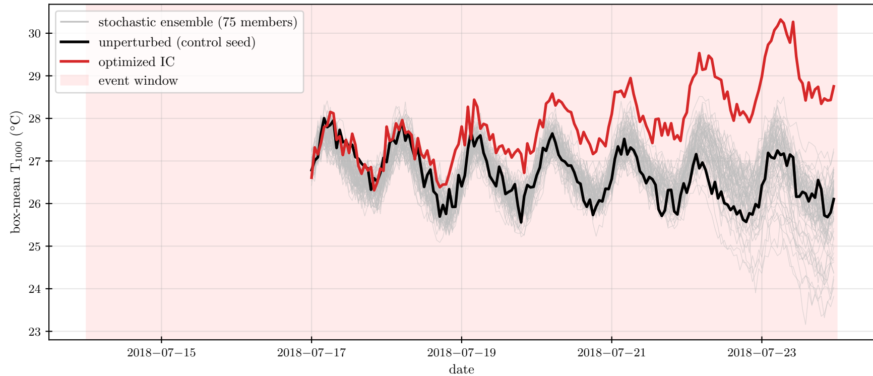
japan_jul2018 storyline vs 75-member ensemble
