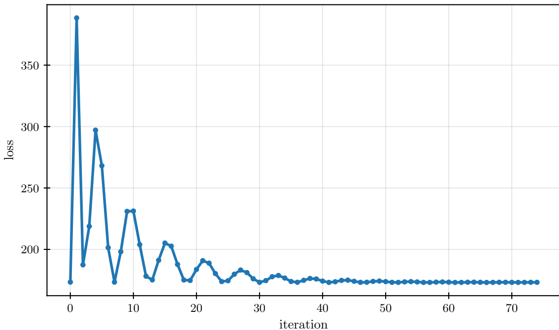
japan_jul2018 IC optimization — loss
