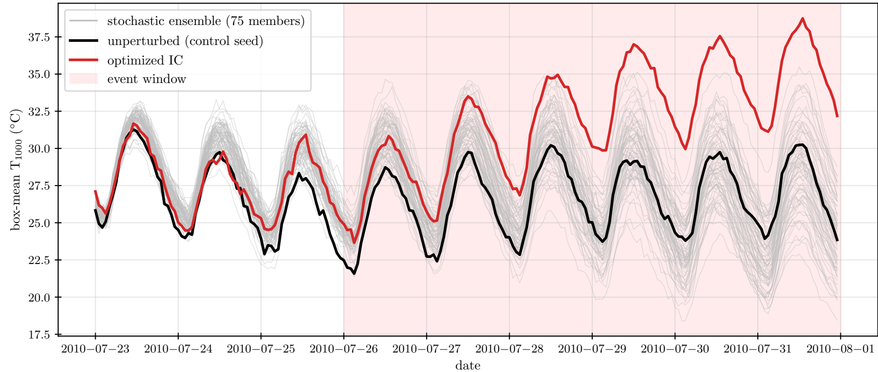
moscow_jul2010 storyline vs 75-member ensemble
