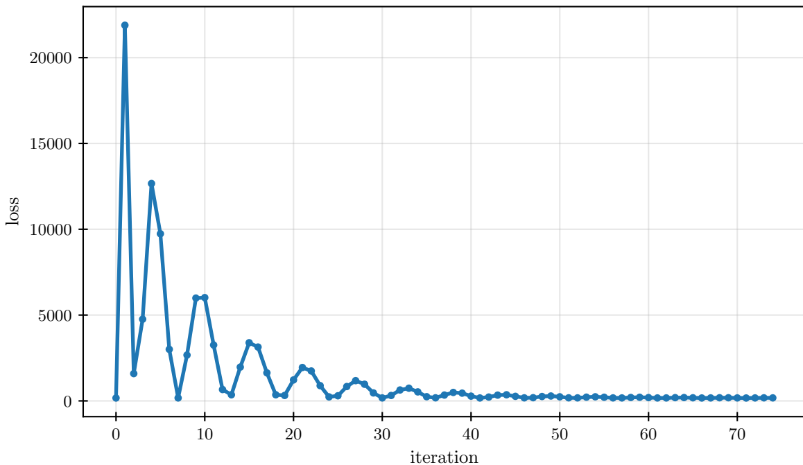
moscow_jul2010 IC optimization — loss
