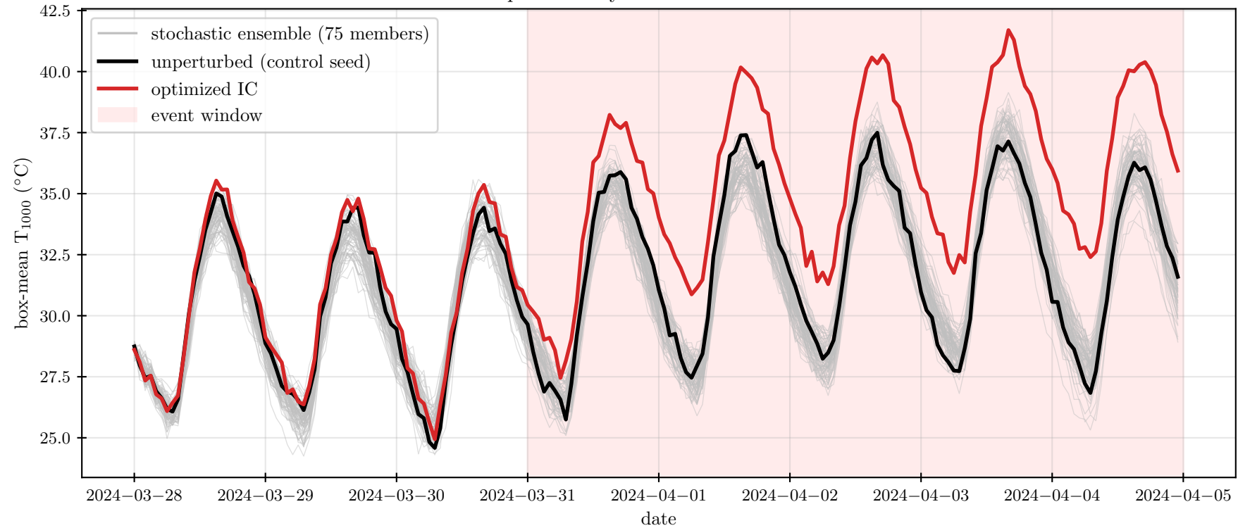
sahel_apr2024 storyline vs 75-member ensemble
