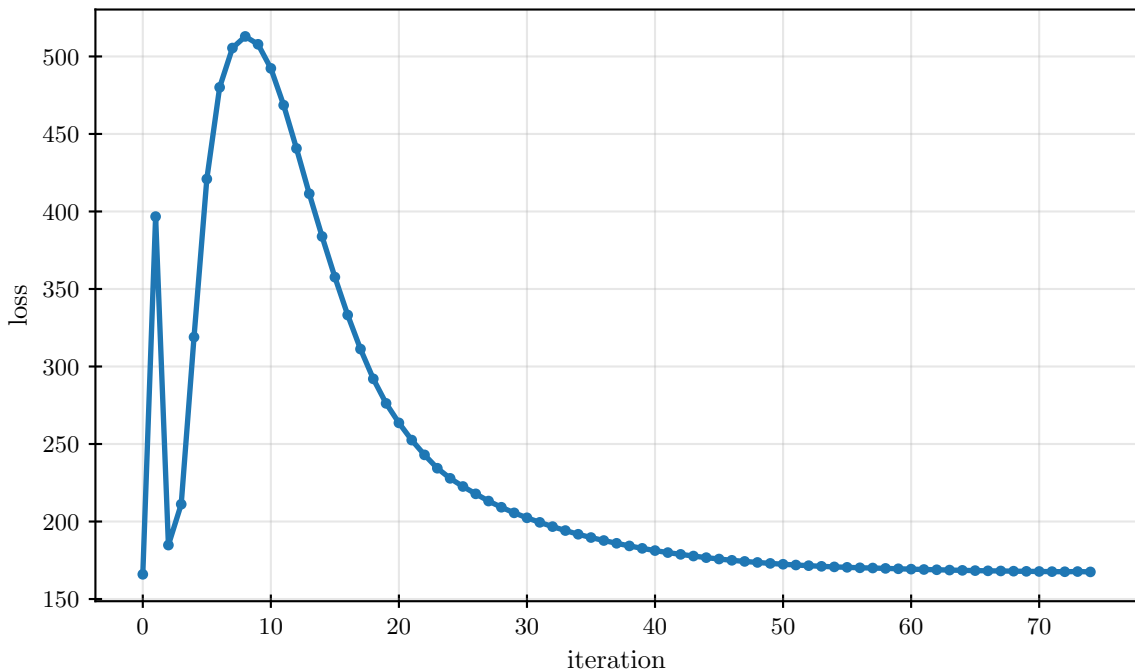
siberia_jun2020 IC optimization — loss
