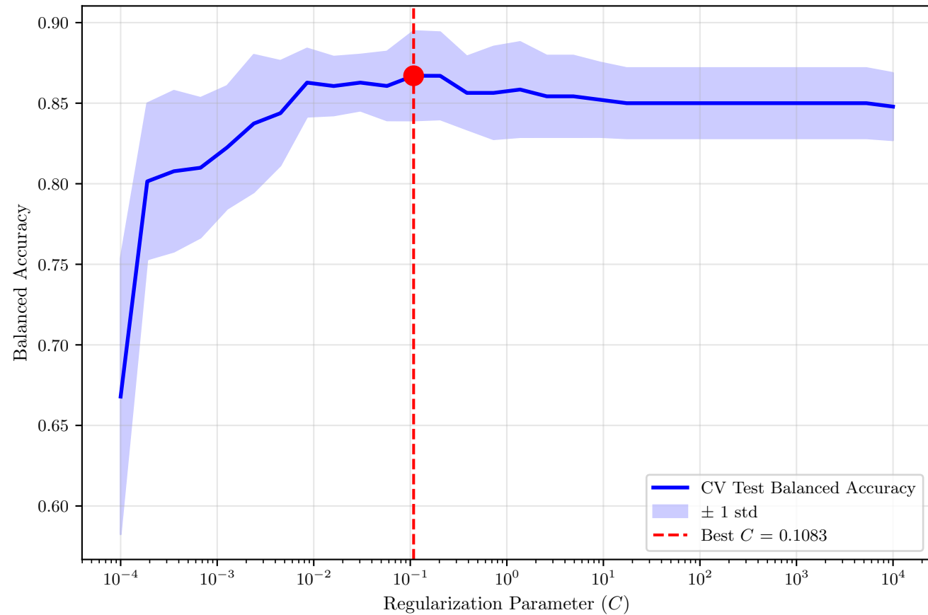
Linear SVM: CV Performance vs C
