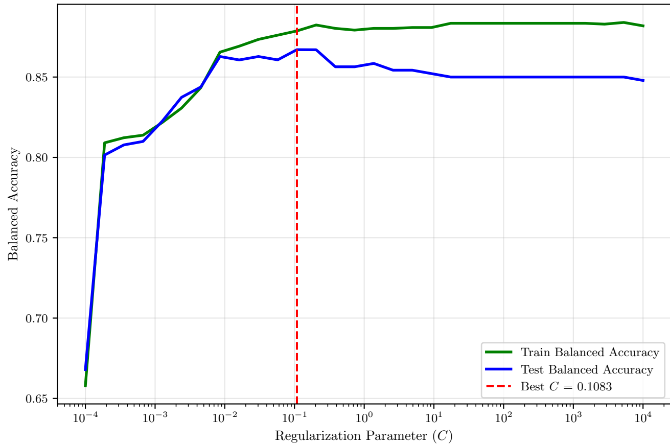
Linear SVM: Train vs Test Performance
