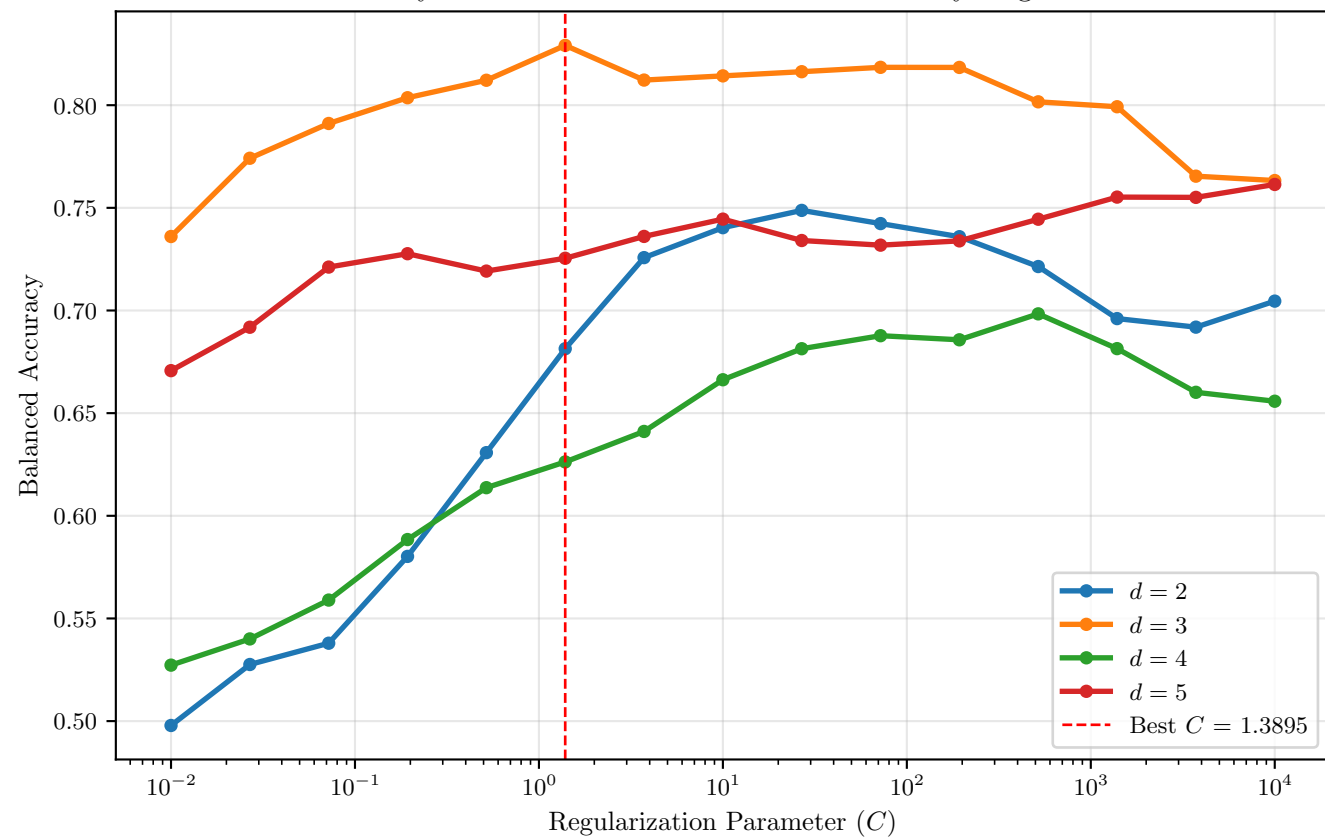
Polynomial SVM: CV Performance vs C by Degree
