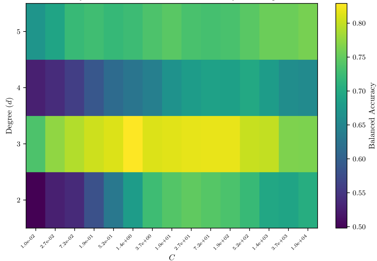
Polynomial SVM: CV Balanced Accuracy Heatmap
