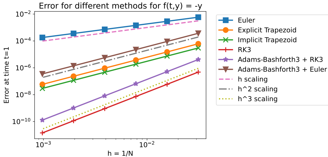
Figure 1: Errors at time t = 1 for a variety of numerical methods for solving y' = f(t, y) as a function of time-step size, 1/N .
