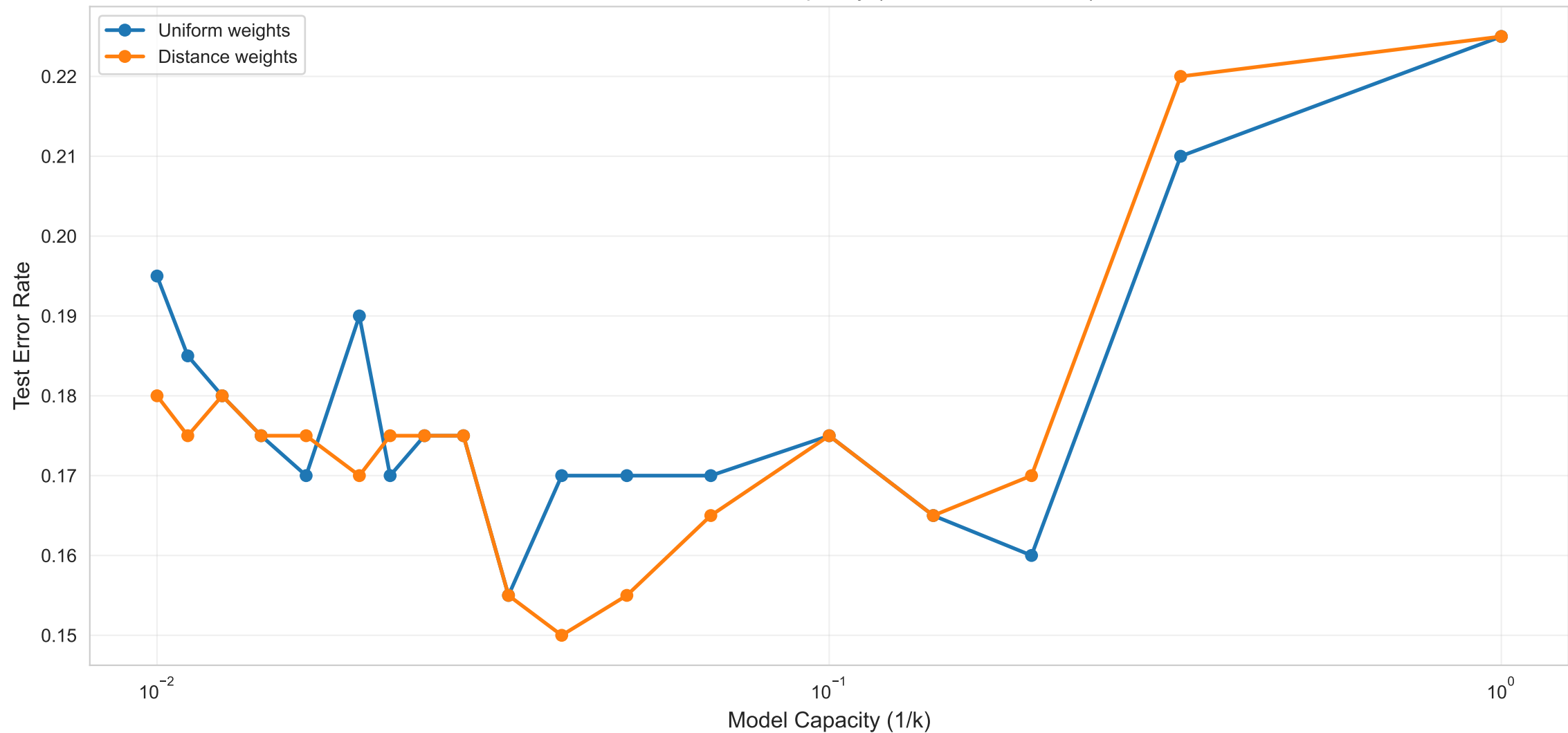
Test Error vs Model Capacity (Euclidean Distance)
