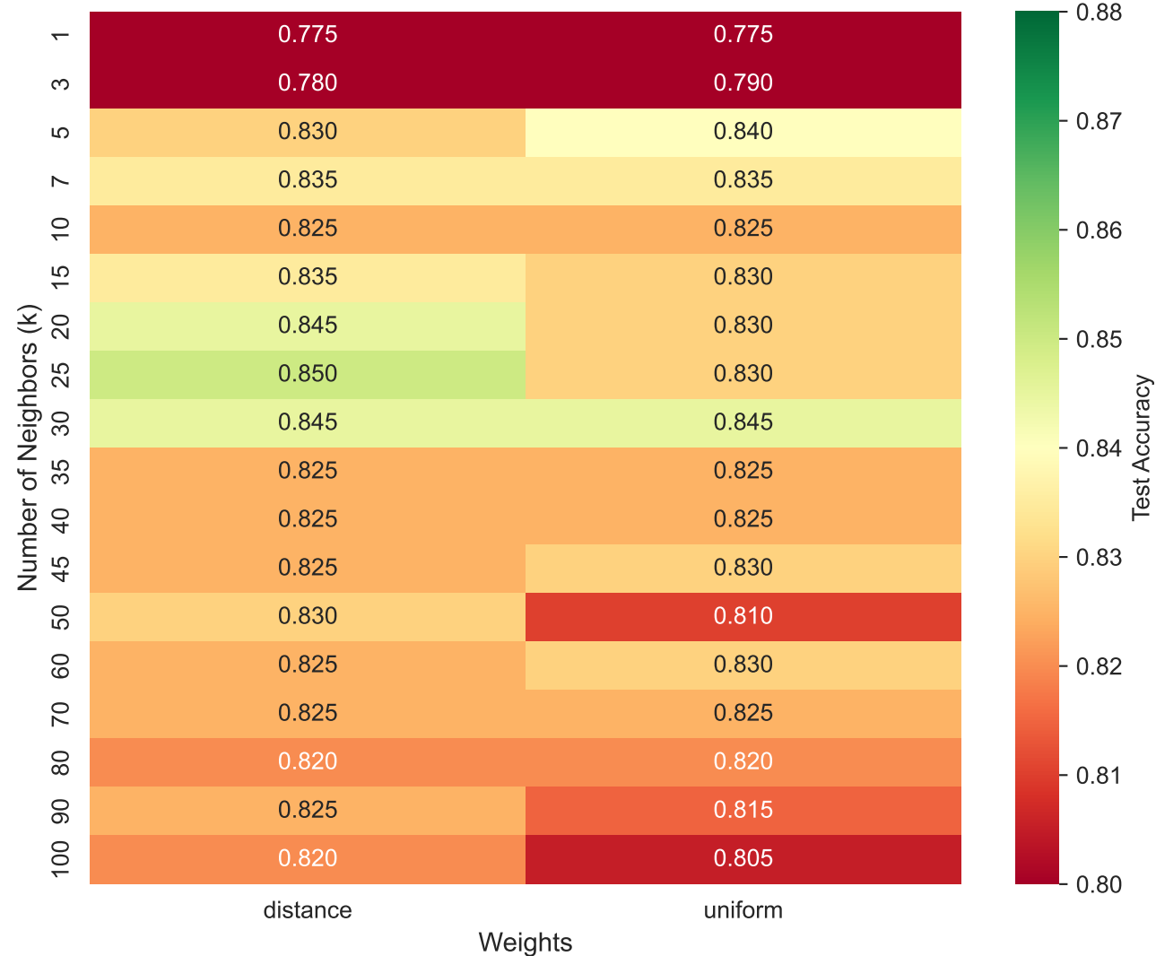
Euclidean Distance
