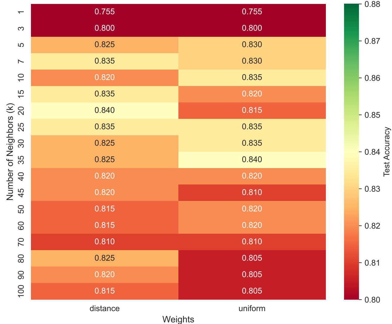
Manhattan Distance
