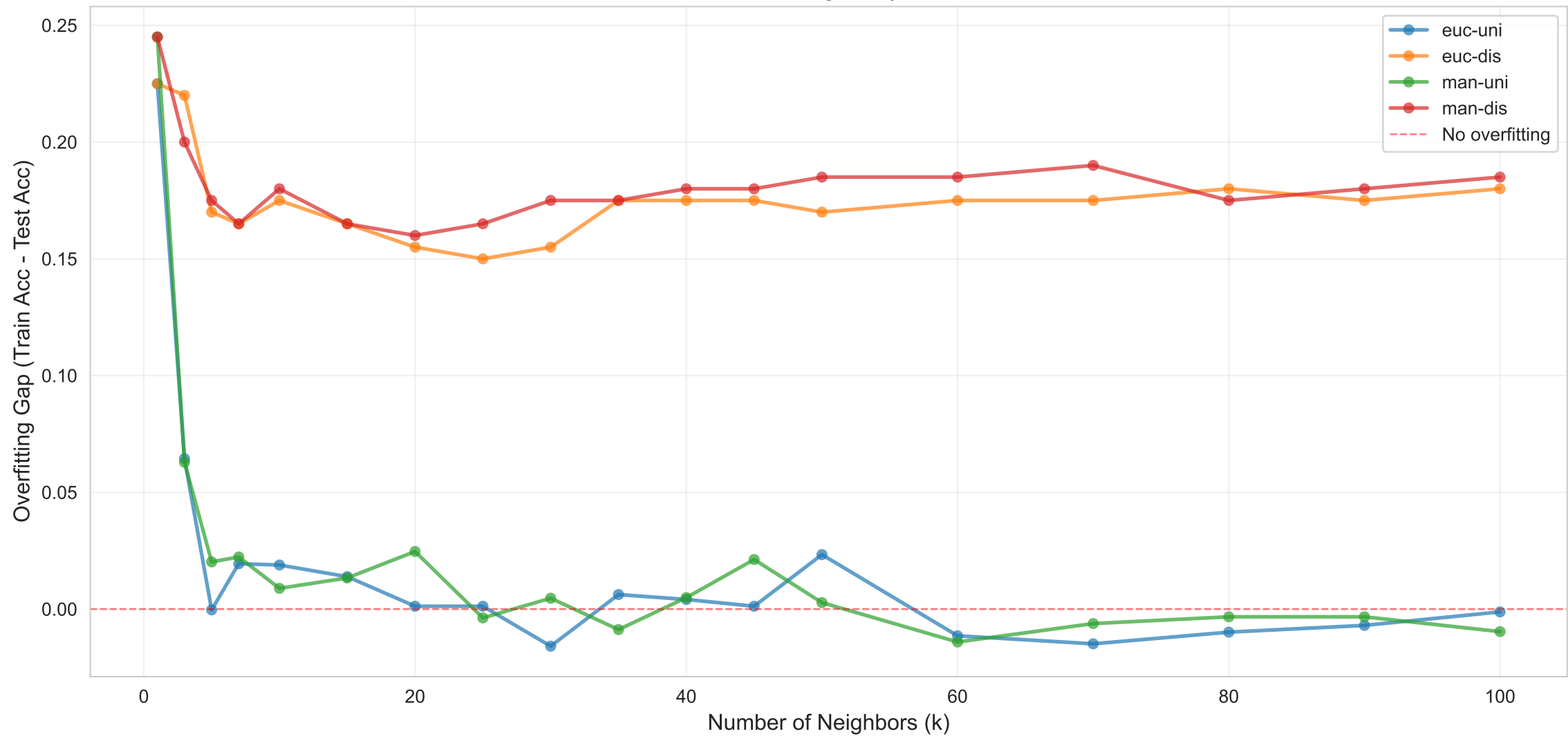
Overfitting Analysis
