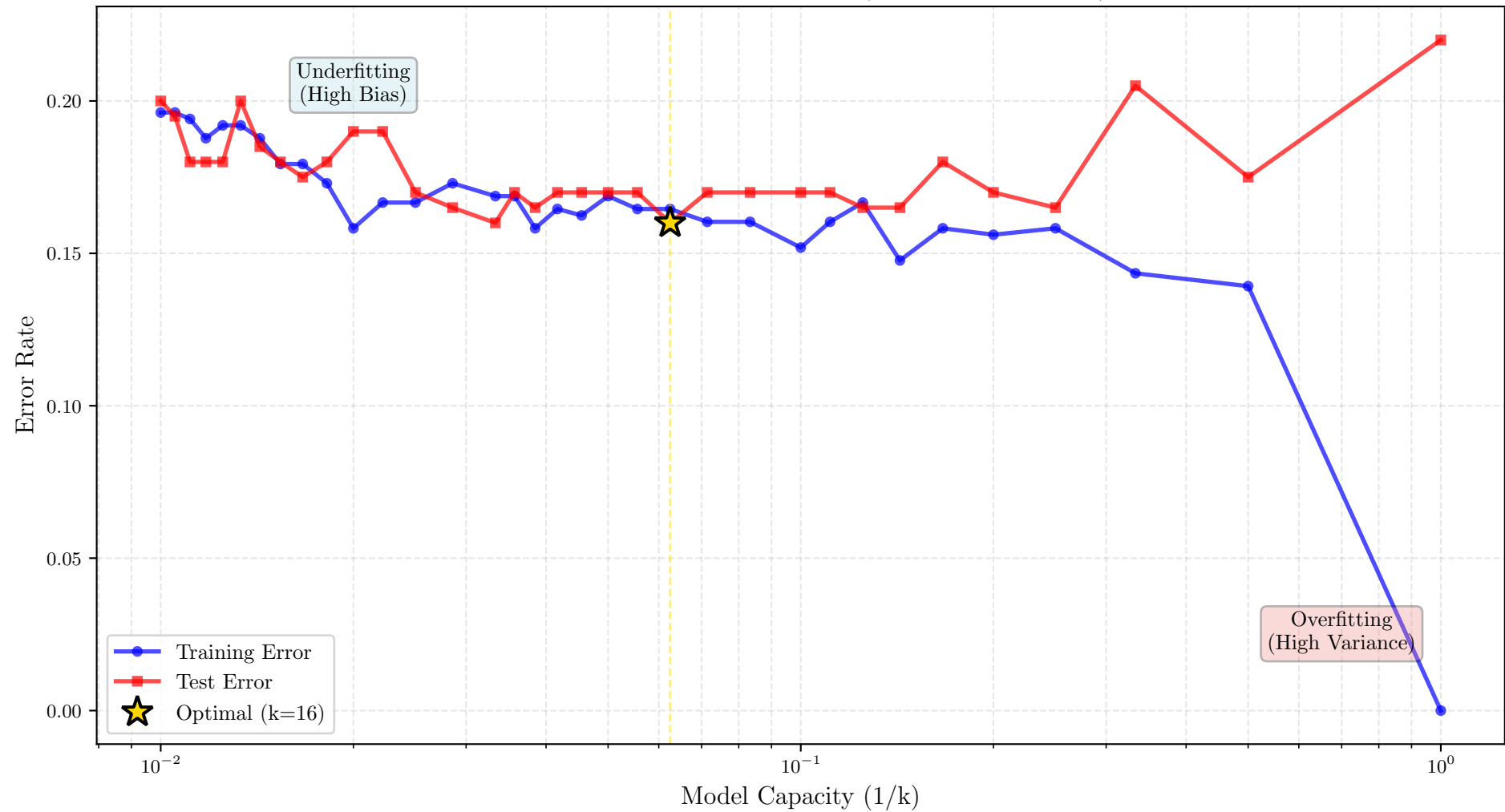
Error Rate vs Model Capacity (Euclidean Distance)
