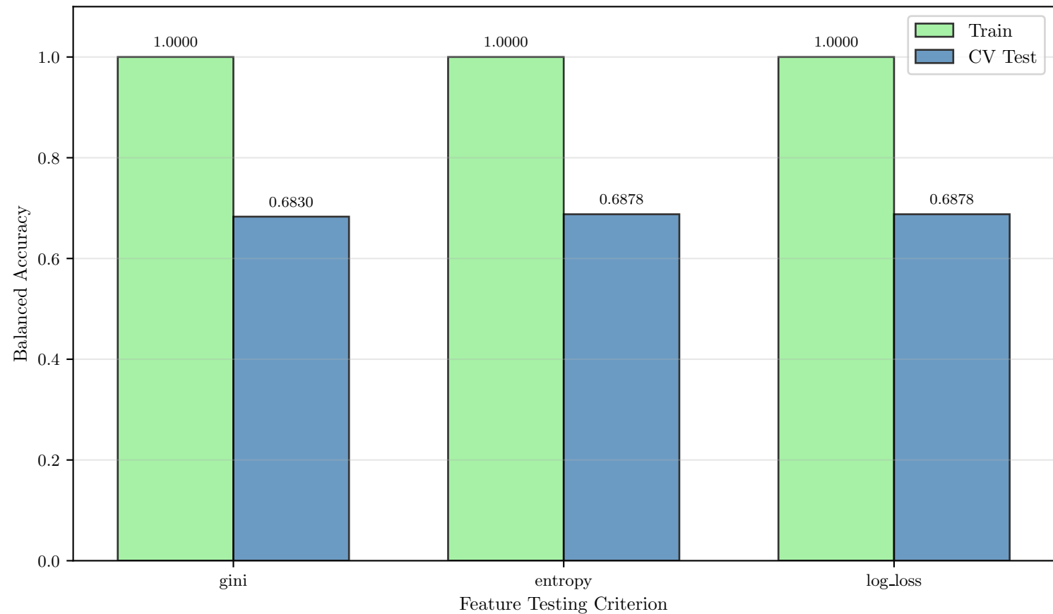
Random Forest: Train vs CV Balanced Accuracy
