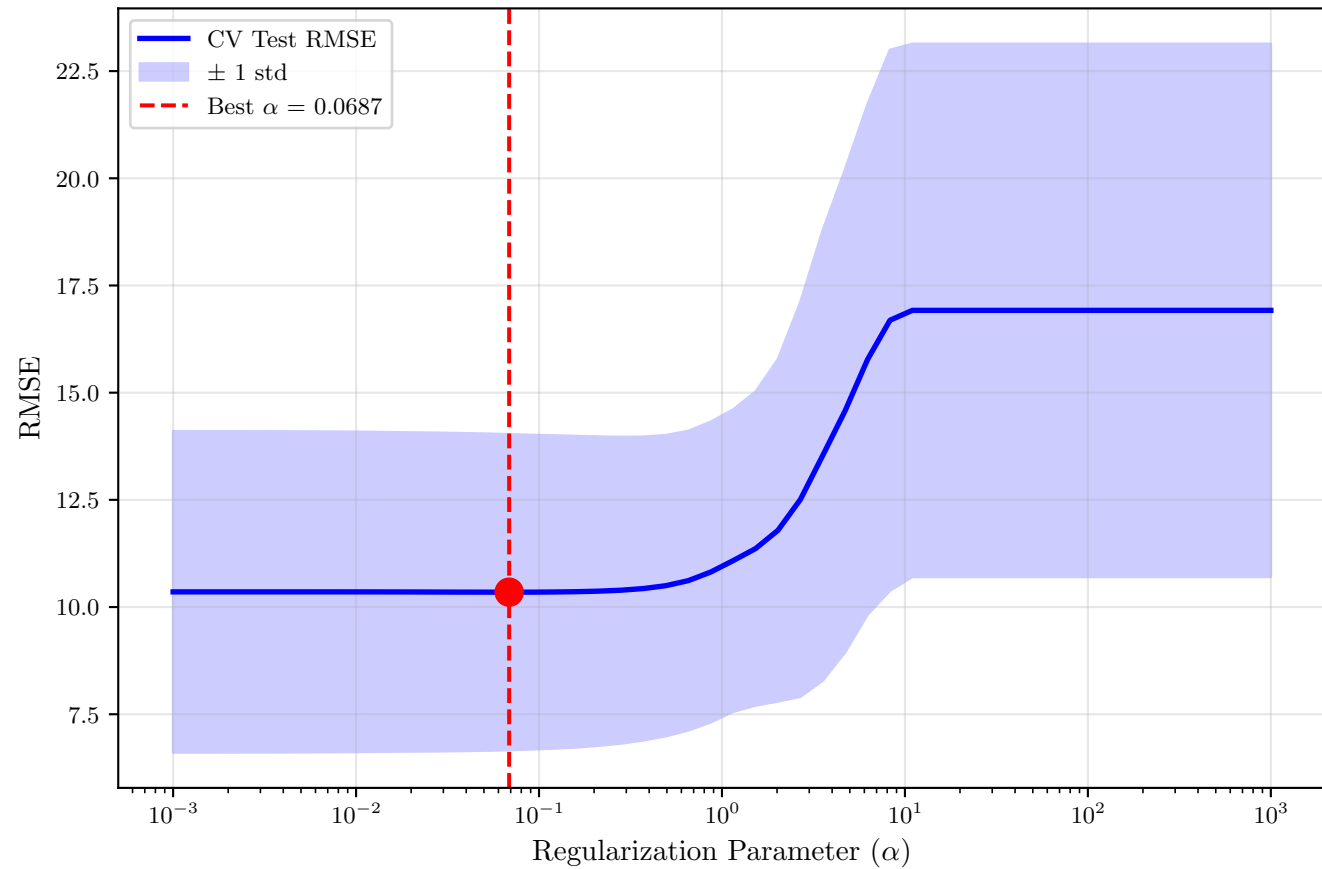
Lasso: Cross-Validation Performance vs \alpha
