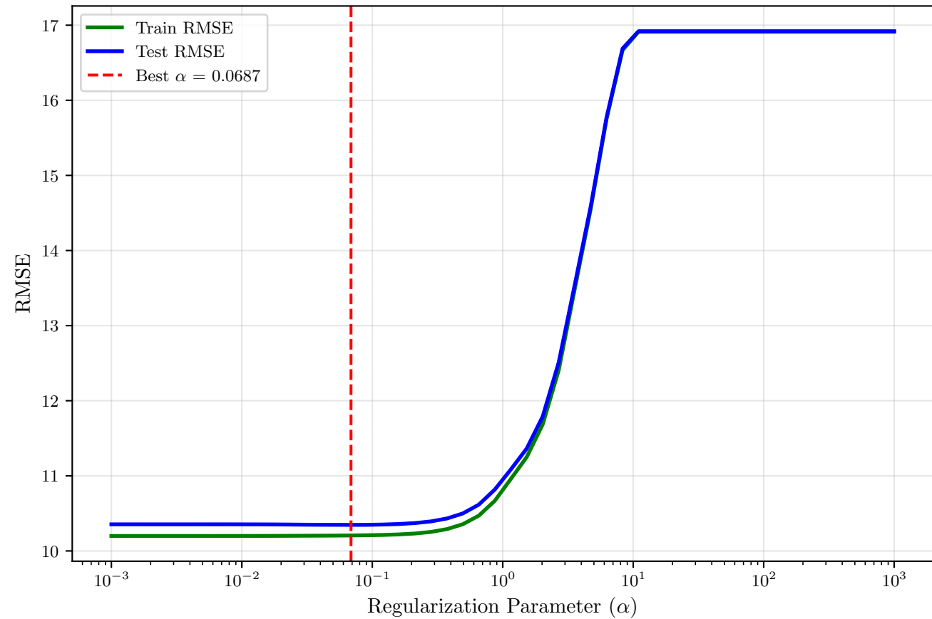
Lasso: Train vs Test Error
