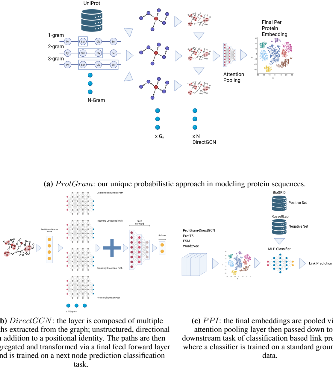
Figure 2: ProtGram – DirectGCN full pipeline.
