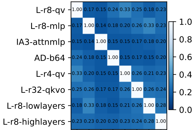
Top-5% overlap
