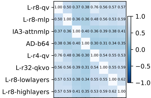
Spearman agreement
