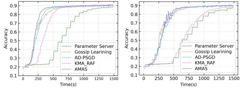
(a) IID-data without dynamic heterogeneity. (b) IID-data with dynamic heterogeneity.
