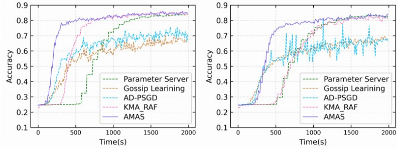
(c) non-IID data without dynamic heterogeneity. (d) non-IID data with dynamic heterogeneity.
