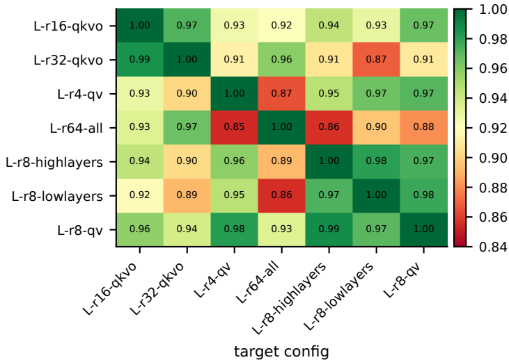
source config
