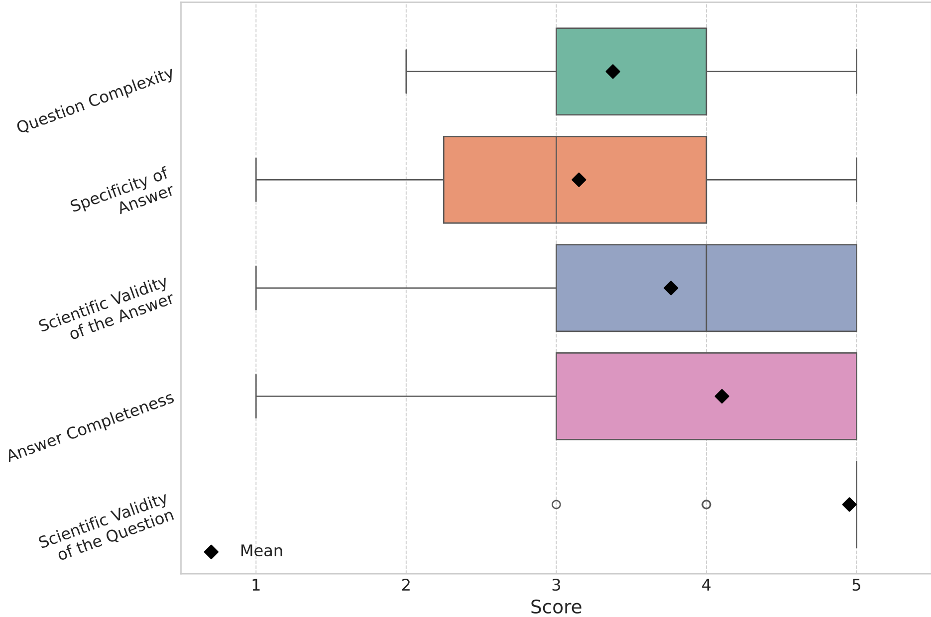
Score Distribution by Evaluation Category
