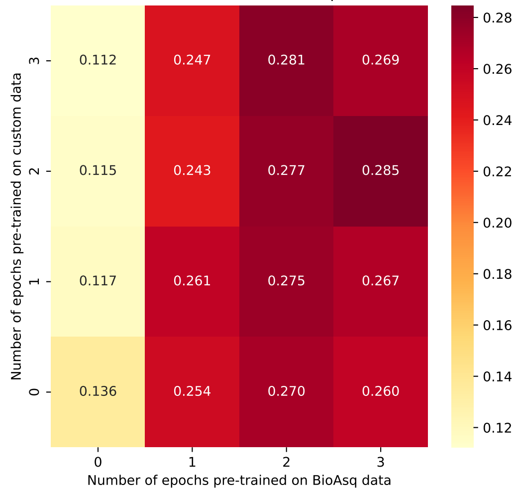
ROUGE-2 Score Heatmap
