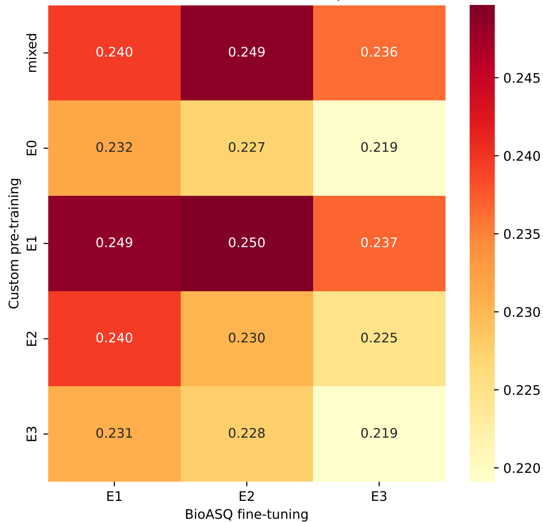
ROUGE-2 Score Heatmap
