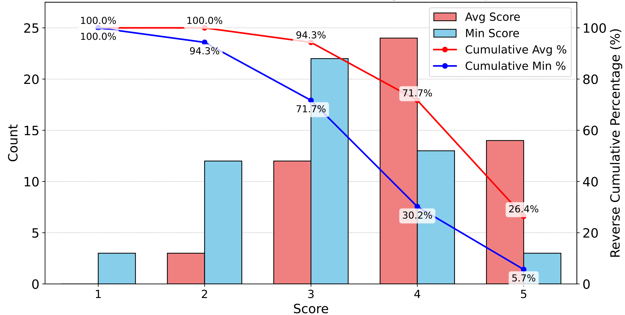
Distribution and Reverse Cumulative Percentage of Scores per Answer
