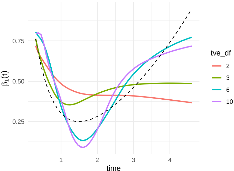
Effect of tve.df on beta1(t)
