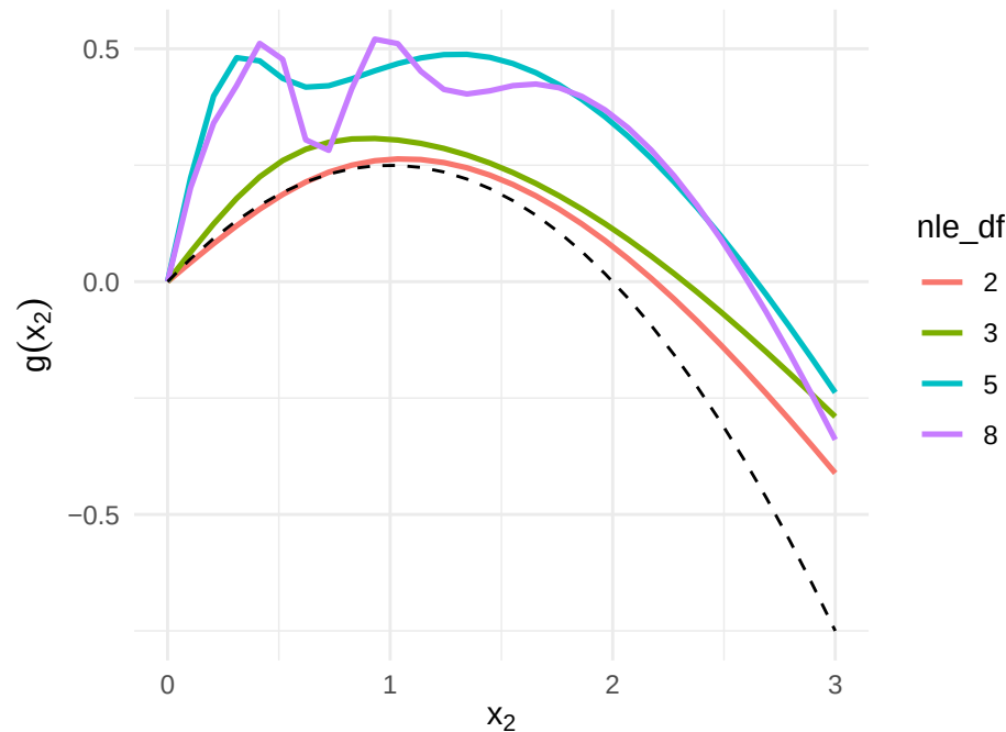
Effect of NLE spline df on g(x2)
