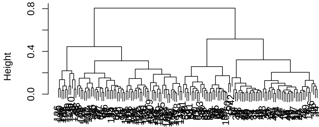
Cluster dendrogram
