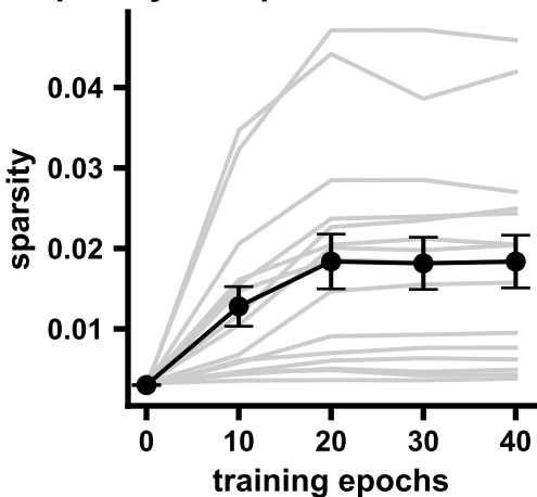
Sparsity vs. Epoch. 10 PCA dims (
