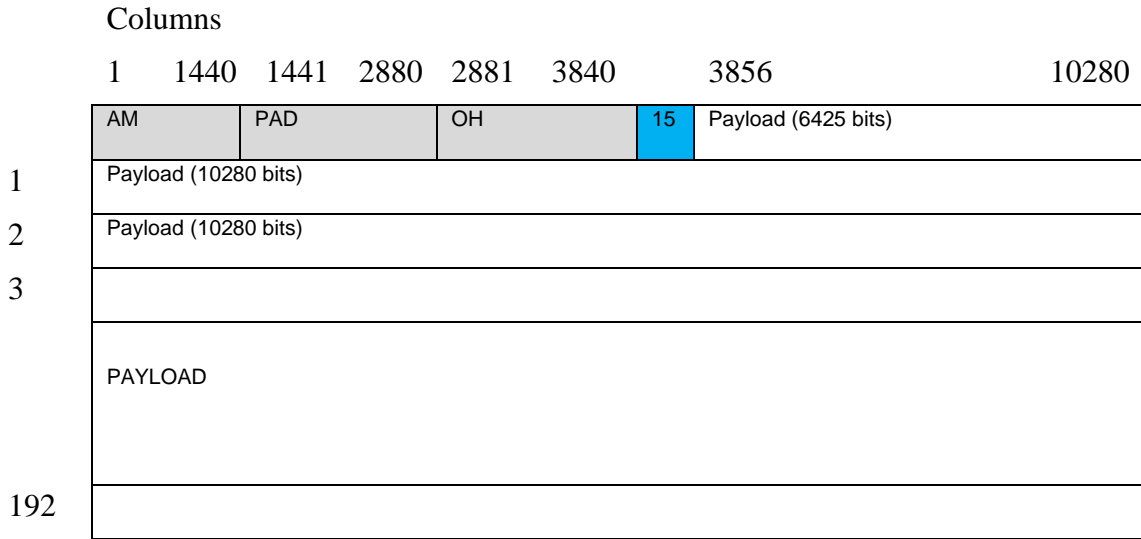
Figure 3-3 – ZR300 Frame
