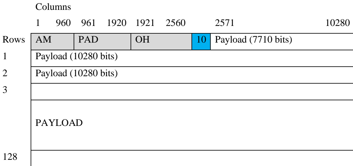
Figure 3-4 –ZR200 Frame
