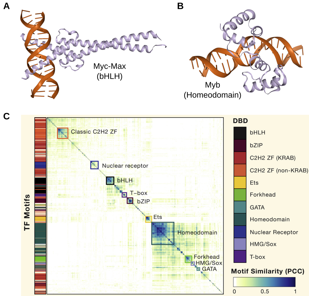
Figure 2.7: Transcription factors with the same DNA binding domains (DBDs) bind similar DNA sequence patterns. A. Homo sapiens TFs Myc and Max binding DNA (Protein Data Bank ID 1NKP). Proteins in purple, DNA in orange. B. Same as A, but Arabidopsis thaliana MYB interaction with DNA (Protein Data Bank ID 6KKS). C. Often TFs with similar DBDs are binding to highly similar DNA motifs. For example, when performing TF motif pairwise comparisons, human TF motifs are grouped according to their DBDs. Adapted from [41].
