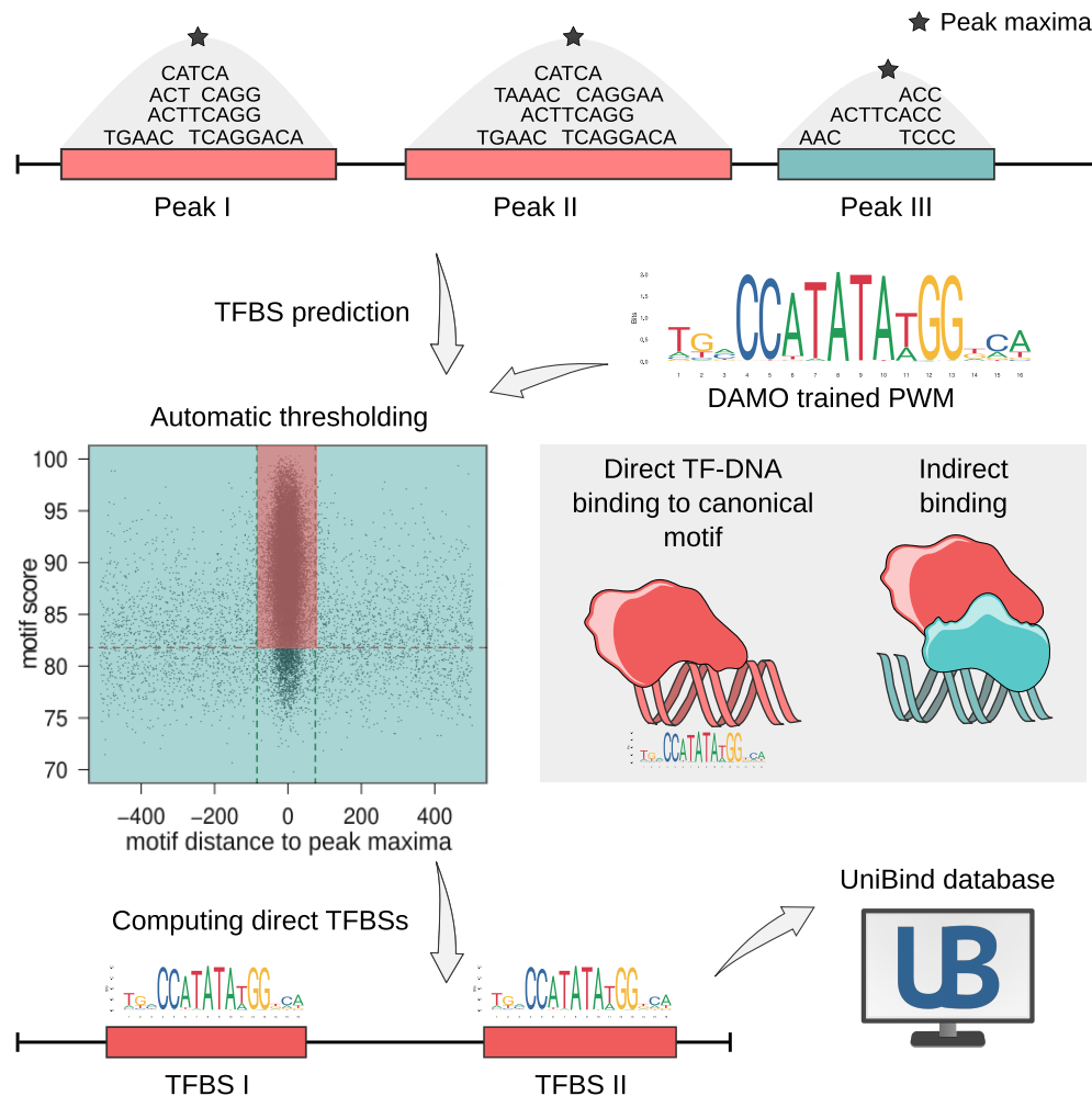
Figure 2.11: An example of combining experimental data with computational models to infer direct TF-DNA interactions. The ChIP-eat pipeline takes ChIP-seq data in peaks and predicts transcription factor binding sites (TFBSs) using the DAMO-trained position weight matrix (PWM) of the profiled TF. During the procedure of automatic thresholding TFBSs that reflect direct TF-DNA binding to the canonical motif (red) are selected from the rest of the predictions that represent indirect or unspecific binding (blue). The final sets of direct TFBSs are collected for each analyzed dataset and compiled into the UniBind database.
