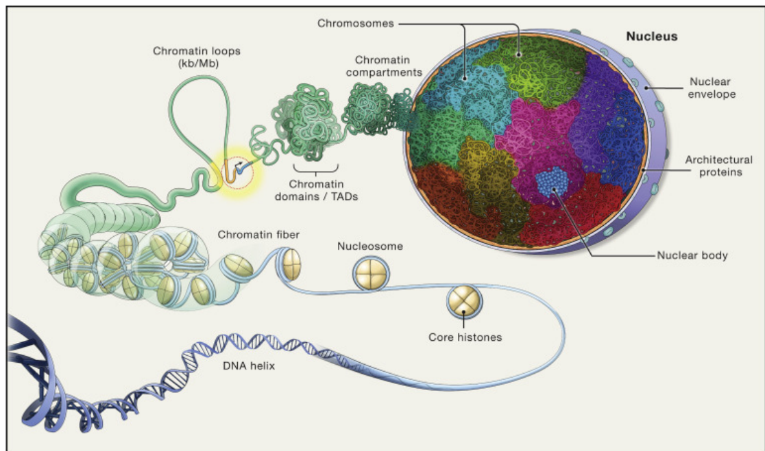
Figure 1.1: Eukaryotic genome organization. Genomic DNA is wrapped up around histones to form nucleosomes - a basic unit of chromatin fibre. Chromatin can form loops that span kilobases (kb) or megabases (Mb) and are essential for gene expression regulation. Bigger stretches of chromatin are organized into domains or topologically associated domains (TADs), which in turn form chromatin compartments to tightly pack everything into the nucleus. Each chromosome usually occupies a territory in the nucleus. The nucleus also contains a nuclear body, architectural proteins and is surrounded by a nuclear envelope. Adapted from [6].
