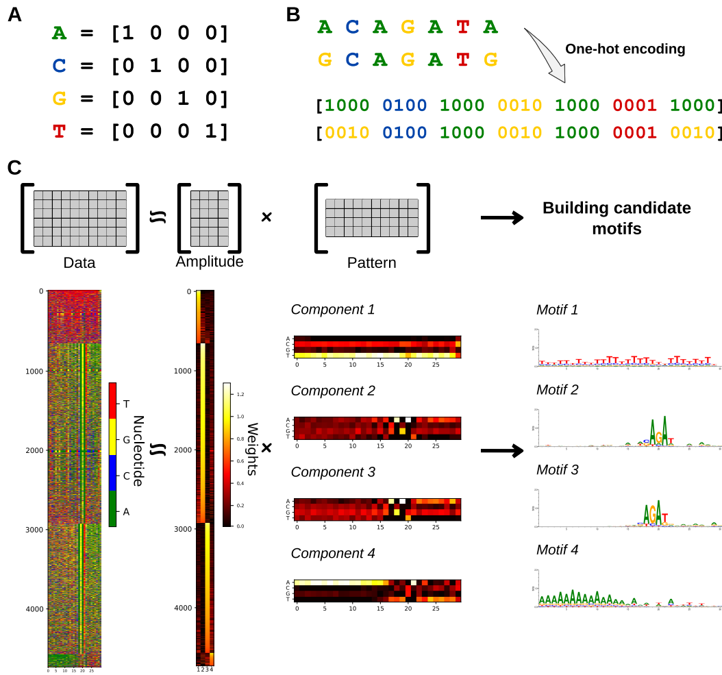
Figure 2.11: Non-negative matrix factorization can be used for DNA pattern discovery in a set of sequences. A. . B. . C. . Adapted from [81].
