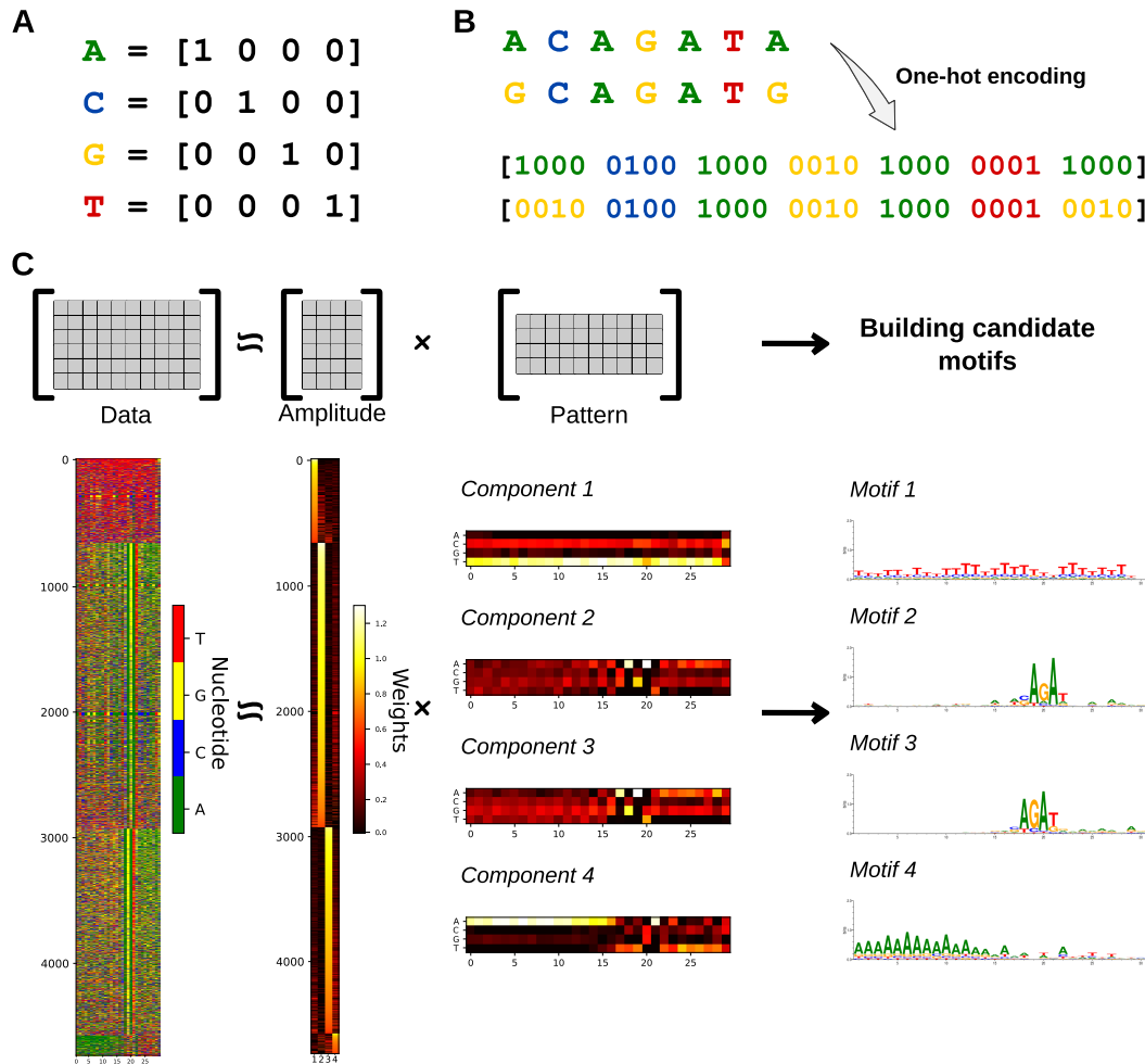
Figure 2.11: Application of non-negative matrix factorization for DNA pattern discovery in a set of sequences. A. Every nucleotide is assigned a unique code. B. DNA sequences are one-hot encoded into an array of ones and zeroes. C. An example of 4 component NMF applied to a set of one-hot encoded DNA sequences (data matrix). The data matrix is factorized into amplitude and pattern matrices. Using the resulting matrices, candidate DNA patterns (motifs) can be built. One motif for each component is built. Adapted from [93].
