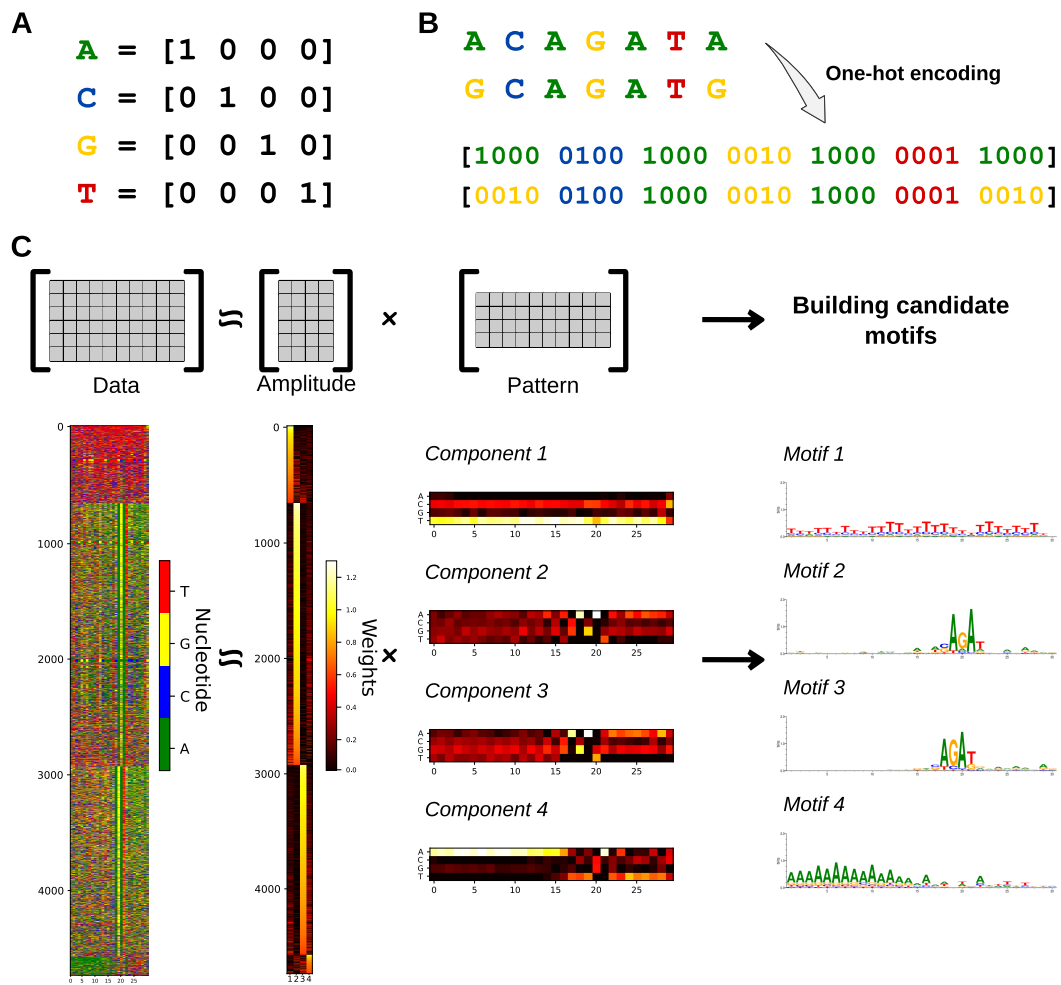
Figure 2.11: Non-negative matrix factorization can be used for DNA pattern discovery in a set of sequences. A. . B. . C. . Adapted from [90].
