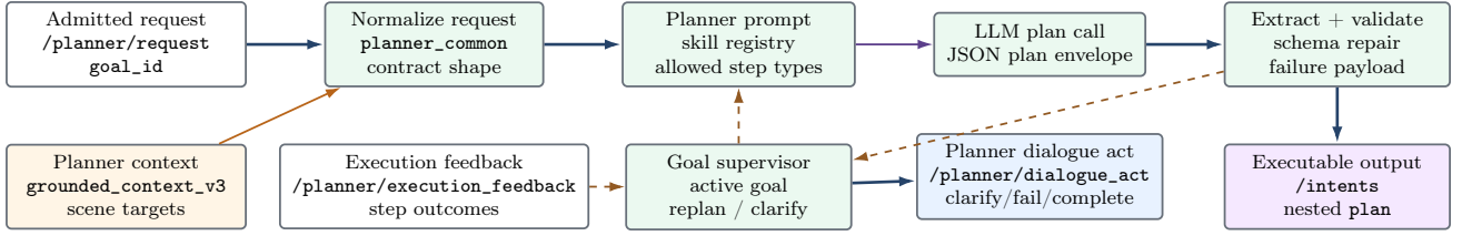
Figure 2: planner_llm node-level view. The planner generates and supervises structured plan envelopes; execution and speech remain downstream responsibilities.
