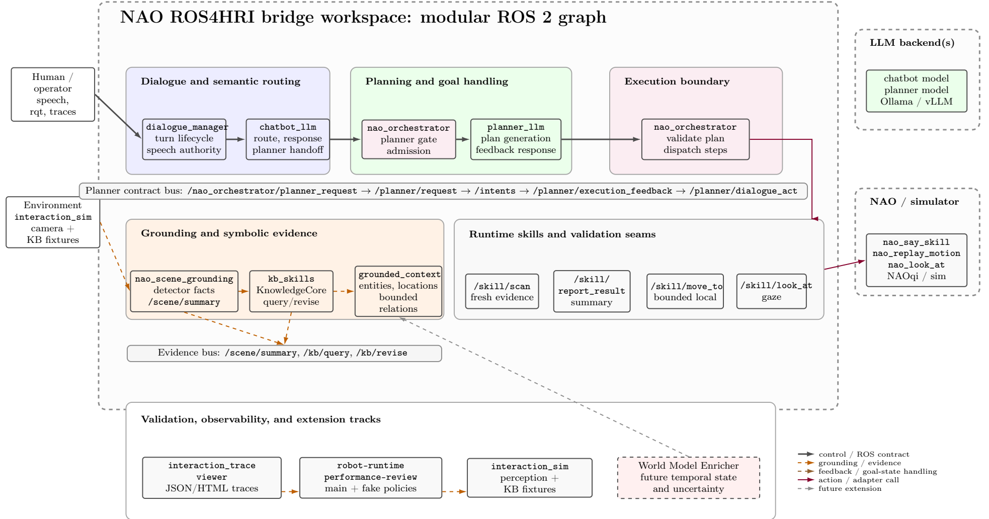
Figure 1: High-level full-stack architecture of the implemented NAO ROS4HRI bridge. The diagram complements the runtime sequence view by emphasizing subsystem ownership, deployment boundaries, ROS contract buses, validation seams, and the future World Model Enricher. The colour coding follows the thesis runtime section: dialogue components are blue, grounding and evidence are orange, planning is green, execution is purple, and skill/adaptor nodes are neutral grey.
