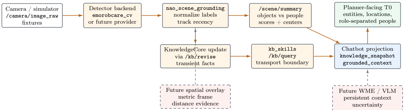
Figure 4: Combined perception and grounding pipeline. Raw detector and KB evidence stays at its owning seams; chatbot and planner consume compact symbolic projections instead of raw perception streams.
