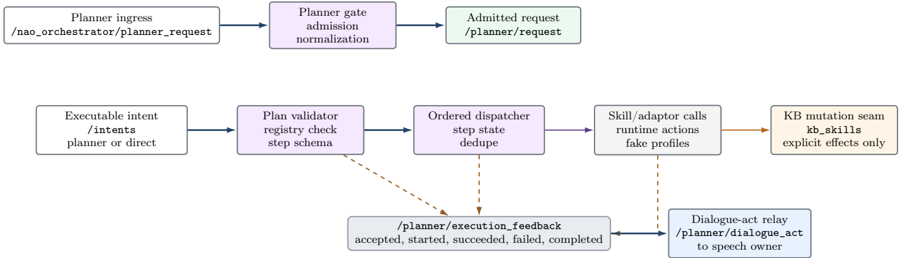
Figure 3: nao_orchestrator node-level view. The orchestrator is the deterministic boundary for admission, validation, dispatch, feedback, and explicit KB mutation routing. It does not plan or produce LLM dialogue policy.
